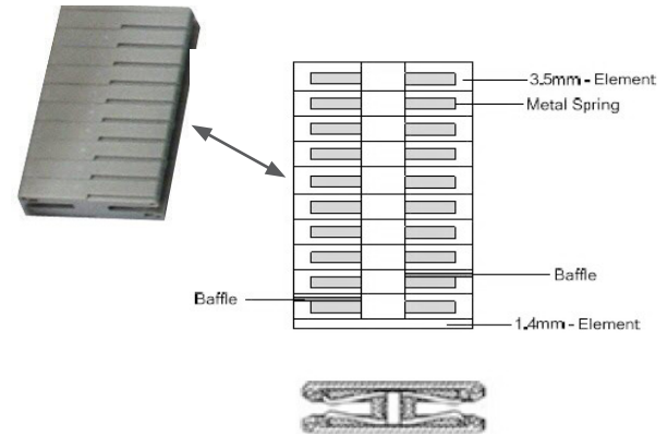
Figure 3: Board-to-Board Connector
